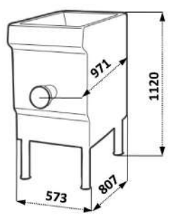
Dimensions TX98 COMPACT
